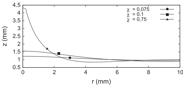
Fig. 8. The ferrofluid–air interface when varying \chi ; for \chi \gtrsim 0.1 , no static hump can form. Increasing \chi results in transition to jetting. For \chi = 0.75 , the dynamic interface stretches until it touches the top boundary of the computational domain, while the interface reaches a static state for \chi = 0.075 and \chi = 0.1 . In all cases L = 6 mm and R_m = 1.5 mm. A secondary instability (or necking that will grow into a pinch-off structure) appears to develop at the tip of the jet for \chi = 0.75 .
