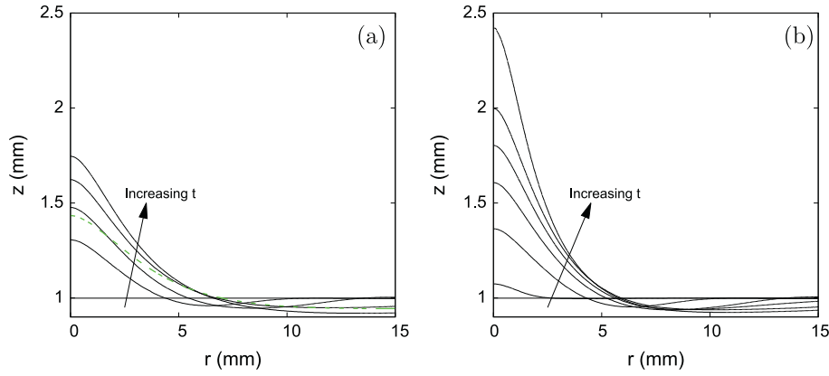
Fig. 6. The ferrofluid–air interface. (a) t = 0, 25, 50, 100, 200, 450 ms (from bottom to top) for L = 5.25 mm. The interface deforms and reaches a static state (green dashed line); the interface undergoes a transient overshoot before settling down to a static shape. The arrow marked “Increasing t ” refers only to the solid (black) curves. (b) t = 0, 5, 25, 50, 100, 150, 200, 248 ms (from bottom to top) for L = 4.95 mm. No sustainable steady interfacial deflection can be obtained and the dynamic interface grows until it touches the top boundary of the computational domain at 250 ms (not shown here). The magnet radius R_m = 3.2 mm and the experimentally fitted value of the magnetic susceptibility \chi = 7.5 \times 10^{-4} . (For interpretation of the references to color in this figure legend, the reader is referred to the web version of this article.)
