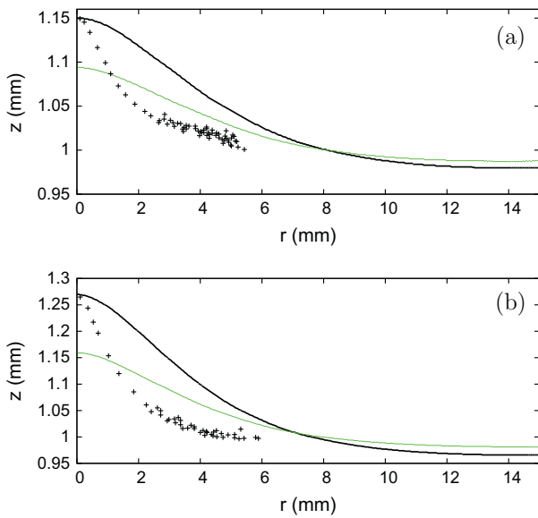
Fig. 4. Experimental data (not pure ferrofluid) from [19] shown alongside our computed steady-state ferrofluid–air interfacial profiles for (a) L = 6.33 mm and (b) L = 5.65 mm. Black solid lines have \chi = 7.5 \times 10^{-4} , chosen to match maximum free surface height to data; green solid lines have \chi = 5 \times 10^{-4} , chosen to fit the data as a whole. The results illustrate the height of the hump and the radial spread of the ferrofluid–air interface. (For interpretation of the references to color in this figure legend, the reader is referred to the web version of this article.)
