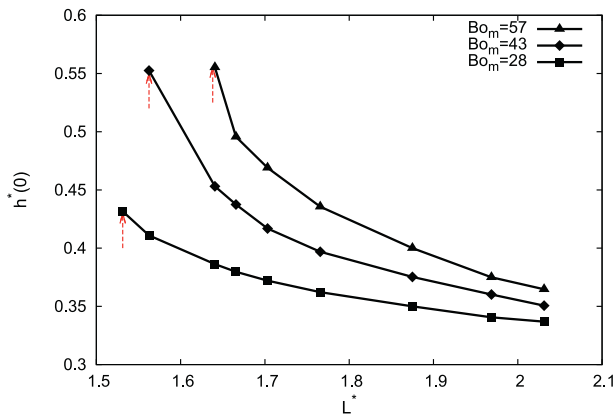
Fig. 9. The maximum interfacial deformation, h^*(0) , versus the non-dimensional distance between the magnet center and the initially flat film, L^* , for various magnetic Bond numbers, Bo_m . R_m = 3.2 mm and \sigma = 0.07 N m ^{-1} . Critical points are marked by red arrows; a smaller L^* will result in no static profiles. (For interpretation of the references to color in this figure legend, the reader is referred to the web version of this article.)
