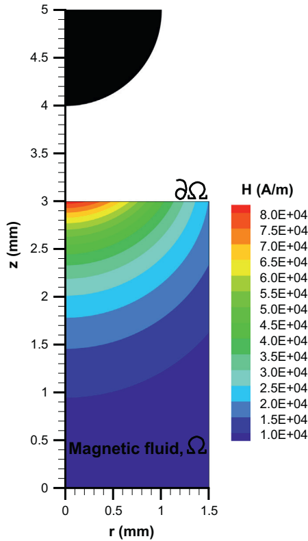
Fig. 2. The computational domain, \Omega , and the computed magnetic field strength, H , with a drawing of a permanent magnet overlaid. The spherical magnet lies outside the computational domain. Number of grid points in the z -direction is N_z = 240 and in the r -direction is N_r = 120 .
