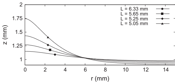
Fig. 5. Static ferrofluid–air interfaces when varying L ; for L \lesssim 5.05 mm, no static hump can form. A decrease in L results in decreasing the radial spreading. The hump also becomes less pronounced with increasing L .
