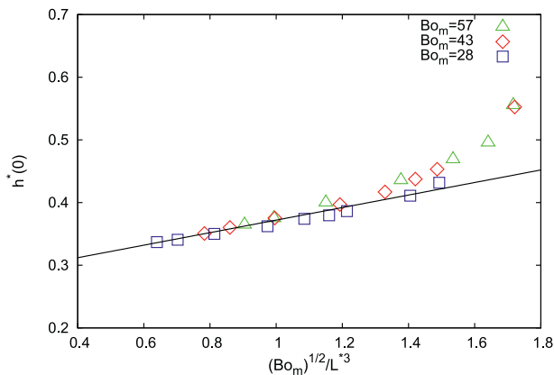
Fig. 10. Non-dimensional maximum interfacial deformation, h^*(0) , plotted against (Bo_m)^{1/2}/L^{*3} for the results in Fig. 9. The solid line is the scaling fit, h^*(0) \propto (Bo_m)^{1/2}/L^{*3} .
