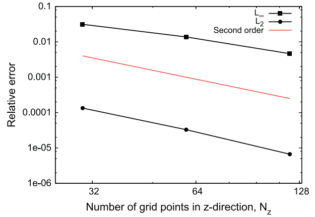
Fig. 3. The convergence of the L_2 and L_\infty relative error norms between the H(r, z) computed at \Delta = L_z/N_z (= L_r/N_r) and at \Delta_{\max} = L_z/240 , for the computational set-up illustrated in Fig. 2.
