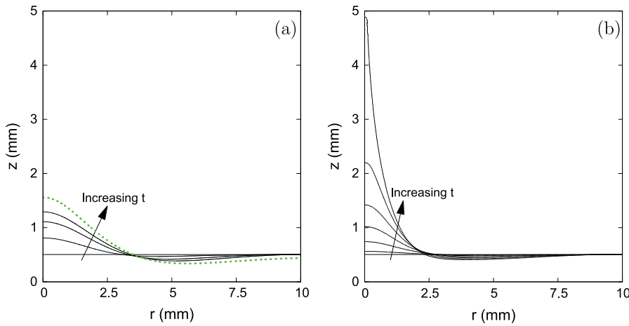
Fig. 7. The ferrofluid–air interface. (a) t = 0, 12.5, 25, 37.5 ms (from bottom to top) for \chi = 0.75 . The interface deforms and reaches a static state (green dashed line) at around t = 150 ms. (b) t = 0, 2.5, 5, 7.5, 10, 12.5, 15 ms (from bottom to top) for \chi = 1.75 . The interface touches the top boundary of the computational domain at around 16 ms (not shown here). L = 6.75 mm and R_m = 1.5 mm. The flat interface shows the initial position of the ferrofluid–air interface. (For interpretation of the references to color in this figure legend, the reader is referred to the web version of this article.)
