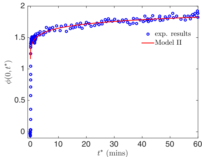
FIG. 14. Evolution of \phi(0, t^*) using Model II (solid red line) and the experimental data of Ref. [12] (results obtained under an electric field applied at time t^* = 0 ). Parameters used to obtain the numerical results are: \lambda_0^* = 0.275 \text{ min}^{-1} and \bar{\beta}_{\text{tol}} = 0.1^\circ .
