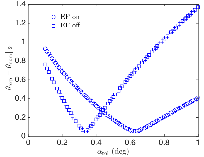
FIG. 8. The error \|\theta_{\text{exp}[5]} - \theta_{\text{num}}\|_2 vs. \bar{\alpha}_{\text{tol}} for electric field on and electric field off scenarios using Model II and the data of Ref. [6].
