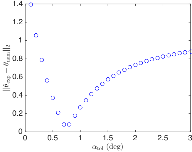
FIG. 11. The error \|\theta_{\text{exp}} - \theta_{\text{num}}\|_2 vs. \bar{\alpha}_{\text{tot}} for electric field off scenario using Model II and the data of Ref. [10].
