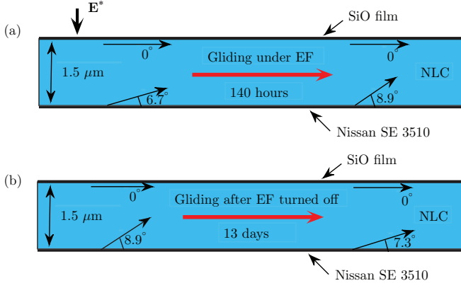
FIG. 3. Schematic summarizing the drift of the easy axis (gliding) at the lower substrate in Ref. [6] (a) during the time of application of an electric field and (b) after the electric field is turned off. Anchoring angles in this and following figures are not drawn to scale.
