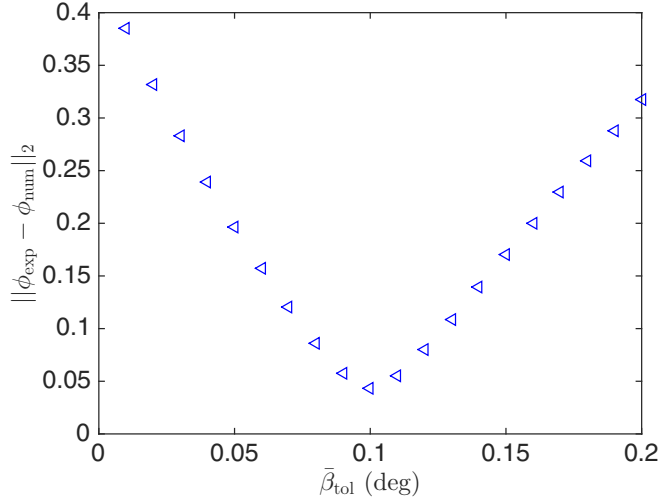
FIG. 13. The error ( \|\phi_{\text{exp}[11]} - \phi_{\text{num}}\|_2 ) vs. \bar{\beta}_{\text{tol}} for electric field on scenario using Model II and the data of Ref. [12].
