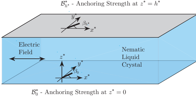
FIG. 2. Sketch showing the setup of the azimuthal model.
