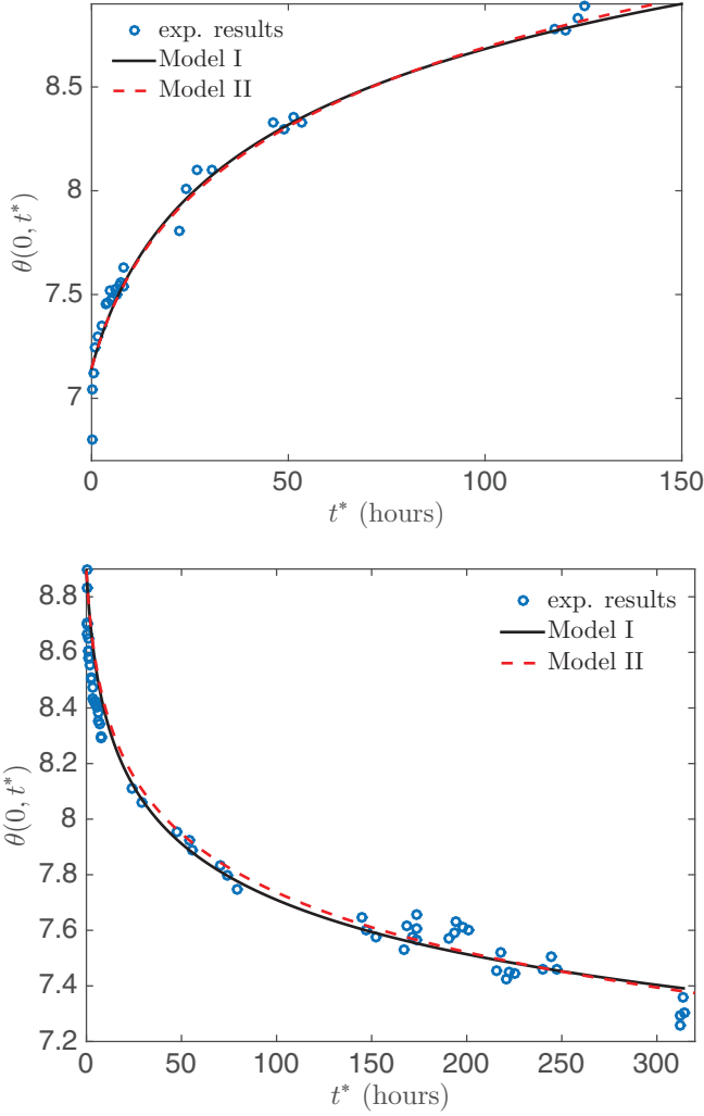
FIG. 9. Experimental results [6] (blue circles) and the results for \theta(0, t^*) using Models I (solid black line) and II (dashed red line) when the electric field is (a) on and (b) off . Parameters used to obtain the numerical results using Model I are: (a) \lambda_0^* = 0.15 \text{ h}^{-1} , n = 12 , \alpha_{\text{tol}} = 8.12^\circ and (b) \lambda_0^* = 20 \text{ h}^{-1} , n = 12 , \alpha_{\text{tol}} = 4.6^\circ . Parameters used to obtain the numerical results using Model II are: (a) \lambda_0^* = 0.15 \text{ h}^{-1} , \bar{\alpha}_{\text{tol}} = 0.63^\circ and (b) \lambda_0^* = 20 \text{ h}^{-1} , \bar{\alpha}_{\text{tol}} = 0.33^\circ .
