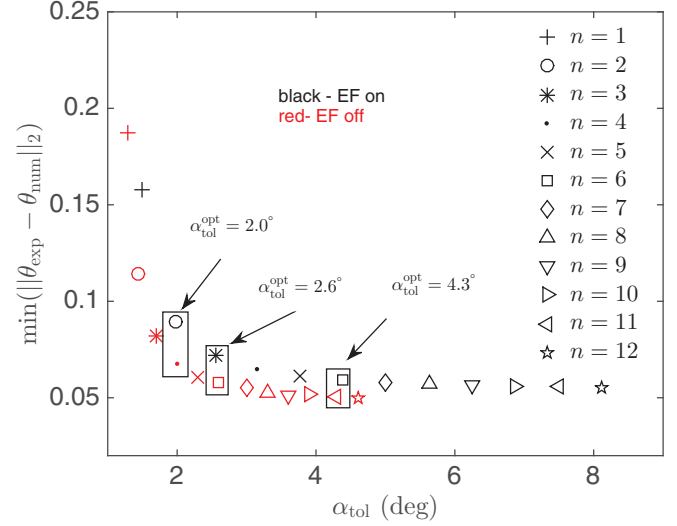
FIG. 6. The error \min(\|\theta_{\text{exp}[5]} - \theta_{\text{num}}\|_2) vs. \alpha_{\text{tol}} for electric field on and electric field off scenarios using Model I and the data of Ref. [6]. Each data point represents different n values.
