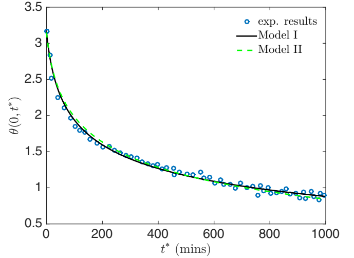
FIG. 12. Evolution of \theta(0, t^*) using Models I (solid black line) and II (dashed green line) and the experimental data of Ref. [10] (blue circles; obtained after the electric field is turned off). Parameters for Model I are: \lambda_0^* = 3.7 \text{ min}^{-1} , n = 6 , and \alpha_{\text{tot}} = 5.4^\circ ; and for Model II, \lambda_0^* = 3.7 \text{ min}^{-1} , \bar{\alpha}_{\text{tot}} = 0.75^\circ .
