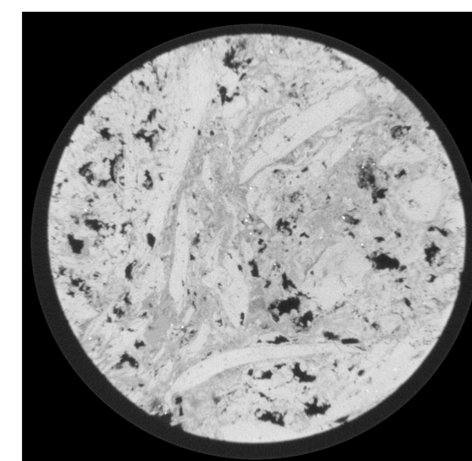
Figure 4: Cross-section of man-made coquina sample, courtesy of Prof. M. Carvalho, PUC-Rio, Brazil. Resolution: 40 microns; dimensions: 1001 x 1024 pixels.
