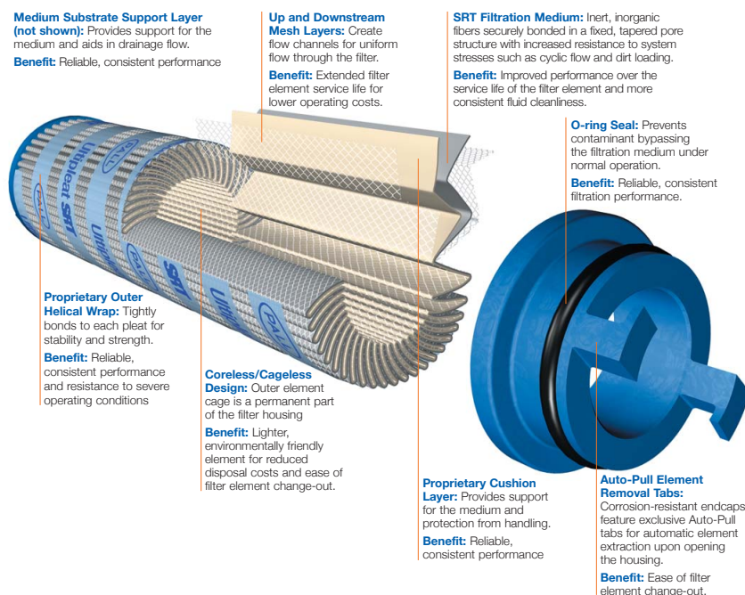
Figure 2.1 Typical geometry of a pleated membrane filter cartridge. Reproduced, with permission, from Pall’s Power Generation Catalog. Source: [1].
